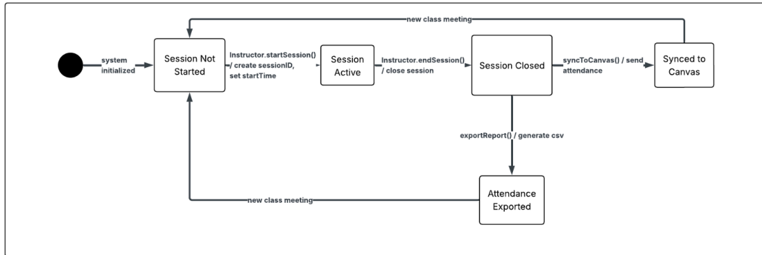
Instructor Session State Machine
