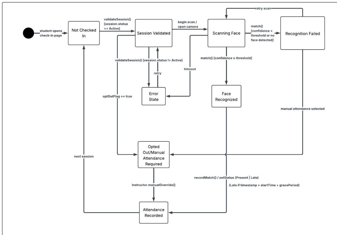
Student Check-In State Machine (Occurs when instructor session is active)
